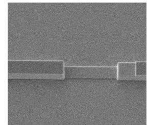
Figure 4. Isolation section, where top layer is locally removed (angled top-view).
